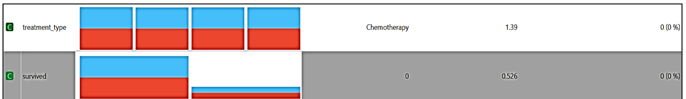
Figure 5: Feature Statistics 3
