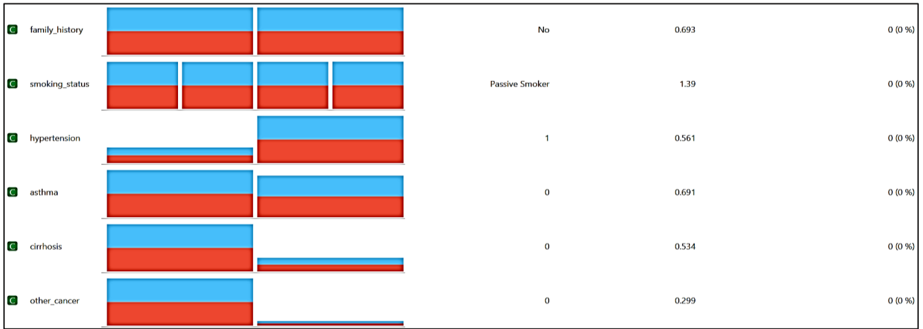
Figure 4: Feature Statistics 2
